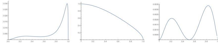
Fig. 8 Figures depict the performance of t -sub-monotone algorithms ( t = 1, 2 ) with expansion factors \beta = 1/(1-p) , as a function of p \in (0, 1) . - Left Figure shows the difference between the competitive ratio achieved by Theorem 4 and the competitive ratio of the 1-sub-monotone algorithm induced by Theorem 3. - Middle Figure shows the behavior of the intermediate turning point \gamma_1 of the 1-Hop of 1-sub-monotone algorithm, compared to expansion factor \beta . The vertical axis equals \gamma_1/\beta = \gamma_1(1-p) , which is shown to be at most 1, as wanted. - Right Figure shows the difference between the competitive ratio achieved by a heuristic 2-sub-monotone algorithm using \beta = 1/(1-p) and the competitive ratio of the 1-sub-monotone algorithm induced by Theorem 3.
