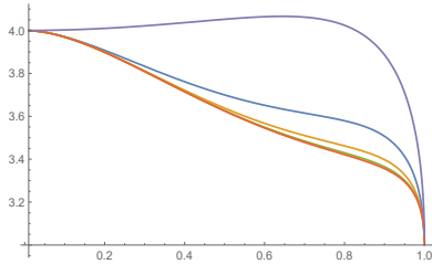
Fig. 3 The vertical axis shows the behavior of the achieved competitive ratio R_t = R_t(p) of various t -sub-monotone algorithms. Purple line corresponds to the monotone algorithm of Lemma 3; that is, when t = 0 . The subsequent improvements for t = 1, 2, 3, 4 are shown in colors blue, yellow, green and red, respectively.
