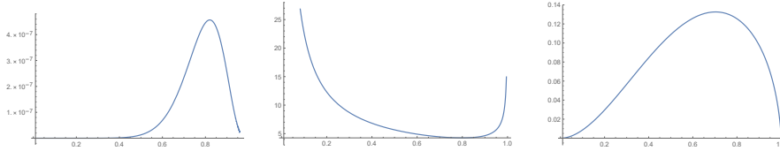
Fig. 9 Figures summarize properties of the limit of pair (\beta_t, R_t) , as defined by Theorem 3, and as t tends to infinity. All the horizontal axes correspond to p \in (0, 1) . - Left figure displays the behavior of R_{10} - \bar{R} , that is the difference between the achieved competitive ratio of the 10-sub-monotone algorithm of Theorem 3 and the ratio \bar{R} one can achieve for arbitrary large values of t . - Middle figure displays the behavior x(p, \bar{R}) , as a function of p , according to which x(p, \bar{R}) > 4 for all p \in (0, 1) , and hence, it is bounded away from 1 as wanted. - Right figure shows that the pair (\bar{\beta}, \bar{R}) satisfies constraint (15). The vertical axis corresponds to (\bar{\beta} - \frac{E}{R/p - F})(1-p)^2 .
