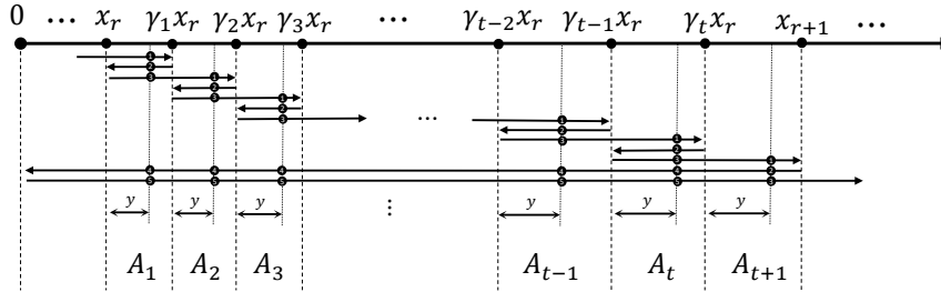
Fig. 2 t -sub-monotone algorithm determined by turning points \{x_i\}_{i \geq 1} and intermediate turning points within hops \gamma_1, \dots, \gamma_t . The figure also depicts all possible intervals A_i , i = 1, \dots, t+1 that the treasure can lie within a t -hop between x_r and x_{r+1} . Possible placements of the treasure are depicted in every interval A_i , along with the first five visitations of the treasure, except the last interval A_{t+1} for which there are only three visitations before the searcher returns to the origin.
