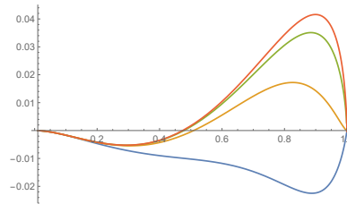
Fig. 4 Figure depicts the behavior of the proposed expansion factors \beta_t = \beta_t(p) for various values of t , as a function of p \in (0, 1) (horizontal axis), that induce the competitive ratios R_t depicted in Figure 3. For the sake of better comparison, the vertical axis is \beta_t(1-p)^2 - (1-p) , which also shows that each expansion factor is more than 1 and less than 1/(1-p)^2 . Colors blue, yellow, green and red correspond to t -sub-monotone algorithms t = 1, 2, 3 and 4, respectively.
