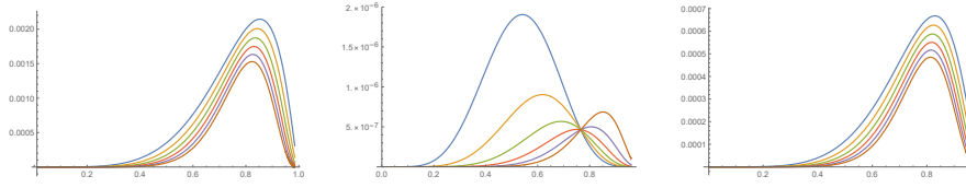
Fig. 7 The figures summarize the behavior of t -sub-monotone algorithms for t = 5, 6, 7, 8, 9, 10 , see colors blue, yellow, green, red, purple and brown, respectively. All the horizontal axes correspond to p \in (0, 1) . - Left figure displays the behavior of the achieved competitive ratio R_t . For each t = 5, \dots, 10 , the vertical axis corresponds to the scaled marginal improvements 4^{t-5}(R_{t-1} - R_t) between two consecutive values of t , which show that the competitive ratio does improve with t , still the improvement is increasingly negligible. The scalar was introduced so that the competitive ratios can be displayed together. - Middle figure displays the behavior of the expansion factors \beta_t that give rise to competitive ratios R_t . For each t = 5, \dots, 10 , the vertical axis is the scaled relative change (1-p)^{11-t}(\beta_t - \beta_{t-1})/\beta_t , where the scalar was introduced to improve comparison. - Right figure shows that the values of \beta_t, R_t chosen, as per the left and middle figures, do indeed satisfy constraint (14) of Theorem 3. The horizontal axis corresponds to (x-y-1)p(1-p)4^{t-5} , where the scalars were introduced so that plots are comparable.
