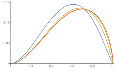
Fig. 6 This figure shows why the choices of \beta_t(p) of Figure 4, that induce the competitive ratios R_t(p) of Figure 3, satisfy constraint (15), as required by Theorem 3. Recall that E, F are functions of p, R_t, \beta_t . For the sake of better comparison, the vertical axis corresponds to \left(\beta_t - \frac{E}{R_t/p-F}\right)(1-p)^2 . Colors blue, yellow, green and red correspond to t -sub-monotone algorithms t = 1, 2, 3 and 4, respectively.
