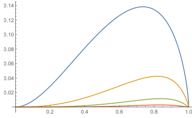
Fig. 5 This figure shows why the choices of \beta_t(p) of Figure 4, that induce the competitive ratios R_t(p) of Figure 3, satisfy constraint (14) as required by Theorem 3. Recall that x, y are functions of p, R_t, \beta_t . For the sake of better comparison, the vertical axis corresponds to (x - y - 1)p(1 - p) . Colors blue, yellow, green and red correspond to t -sub-monotone algorithms t = 1, 2, 3 and 4, respectively.
