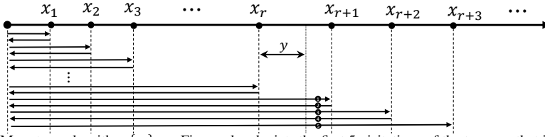
Fig. 1 Monotone algorithm \{x_i\}_{i \geq 1} . Figure also depicts the first 5 visitations of the treasure that is placed at x_r + y .
