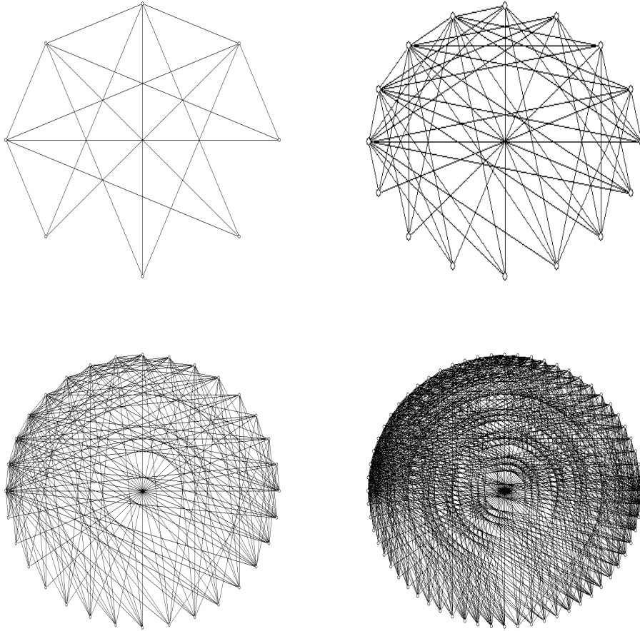
FIGURE 1. The evolution of the ILT model with G_0 = C_4 , for t = 1, 2, 3, 4 .
