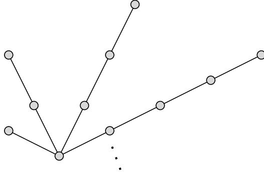
FIGURE 2. The tree T_\omega .
